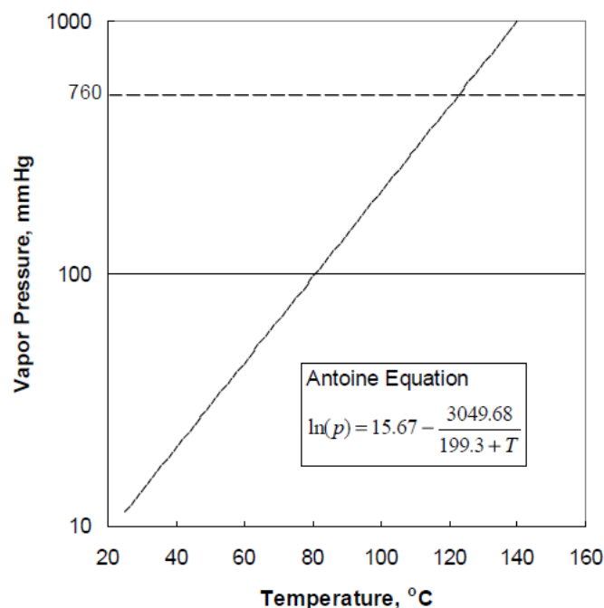
Figure 1. Vapor Pressure of Dytek® HMI
